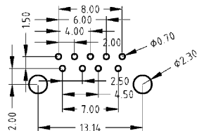
CONNECTOR FRONT EDGE REFERENCE PCB LAYOUT
