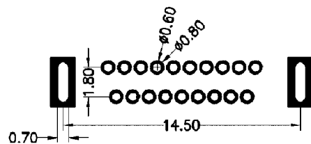
RECOMMENDED PCB LAYOUT (180° DIP)
